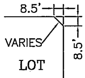
TYPICAL CORNER LOT CHAMFER DETAIL NO SCALE
